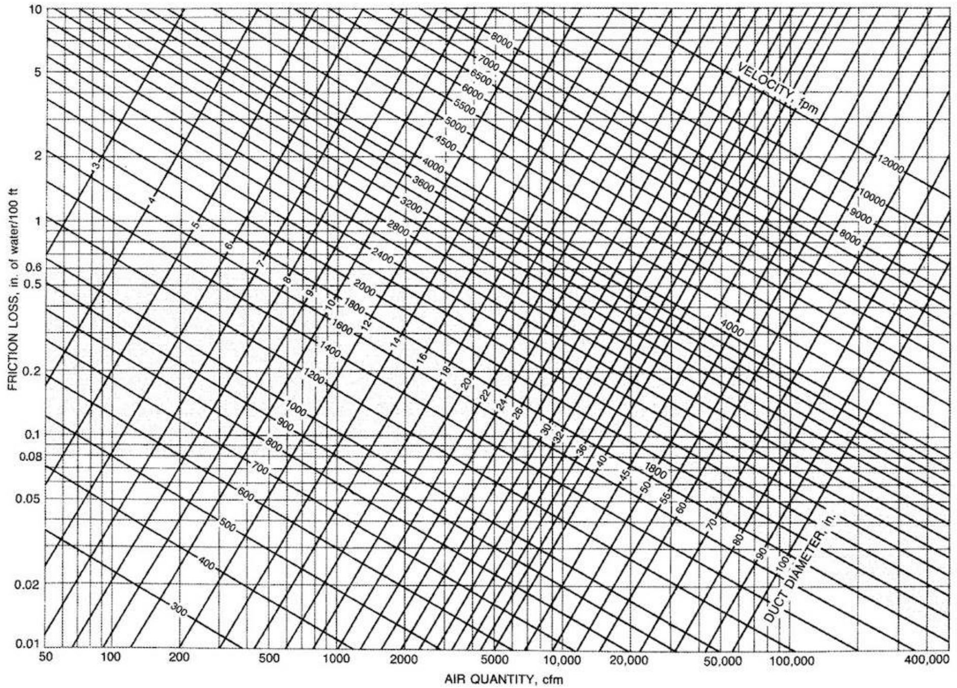
Fig. 9 Friction Chart for Round Duct ( \rho = 0.075 \text{ lb}_m/\text{ft}^3 and \epsilon = 0.0003 \text{ ft} )
